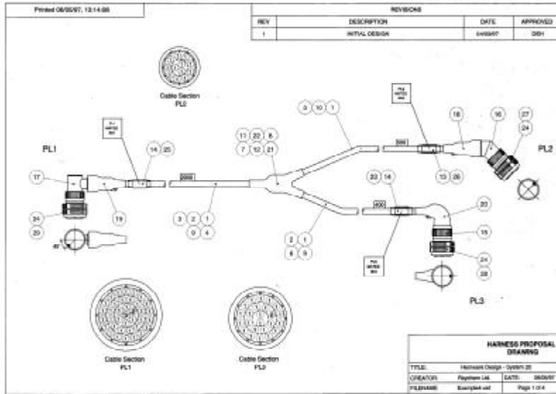
Figure 2. Typical harness drawing generated by HamWare.
